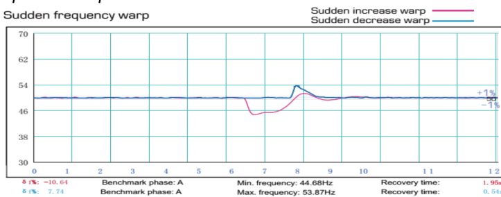
Sudden frequency warp
