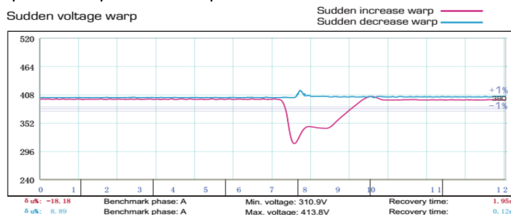
Sudden voltage warp
